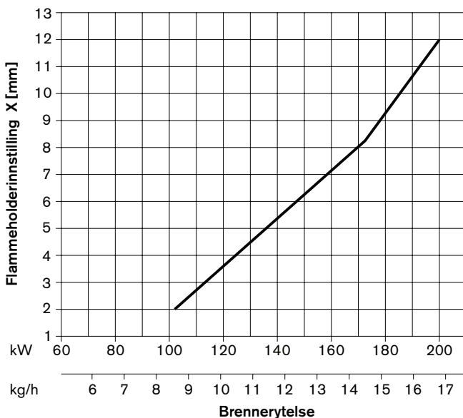
Grunninnstillingsverdier flammeholder WL20/2-C, utf. Z
